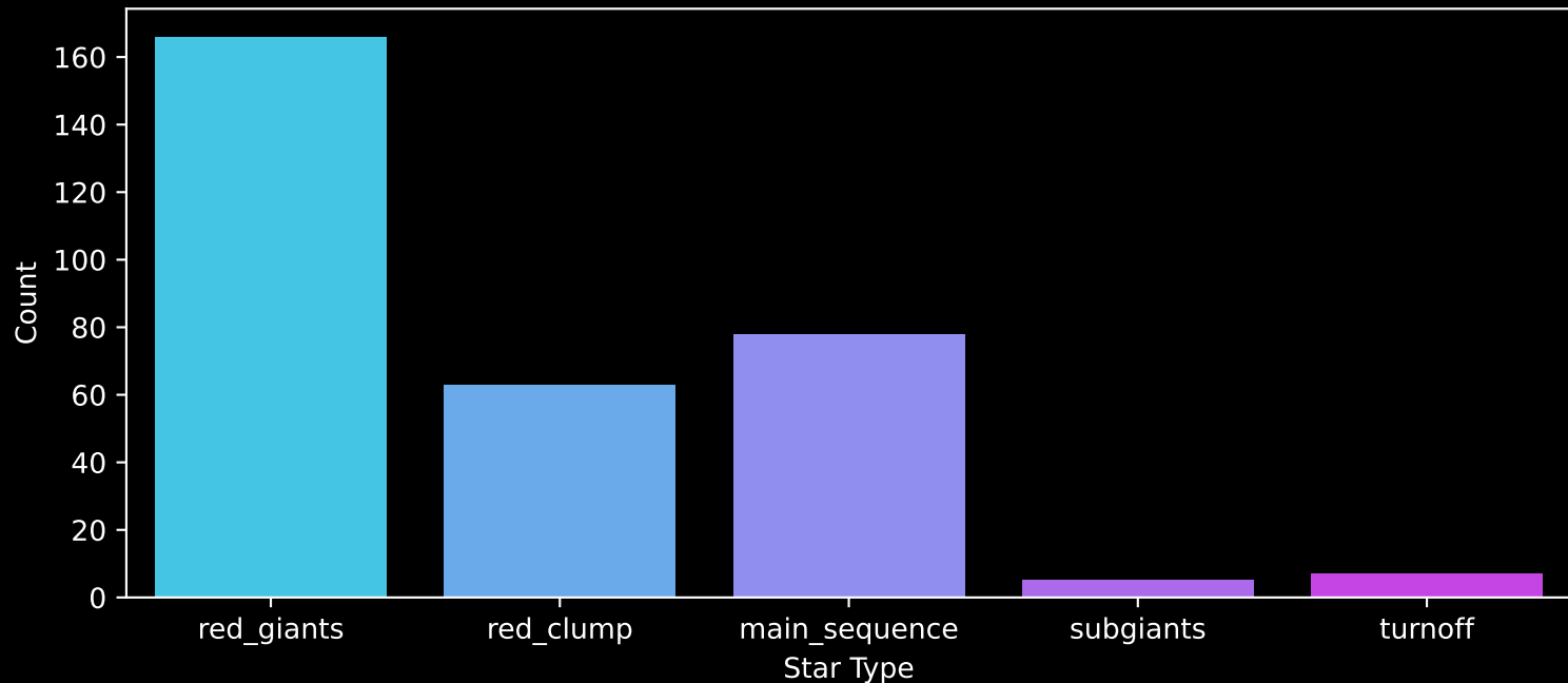
APOGEE DR17 Field: [214+18_btx] Count plot of Star Type
