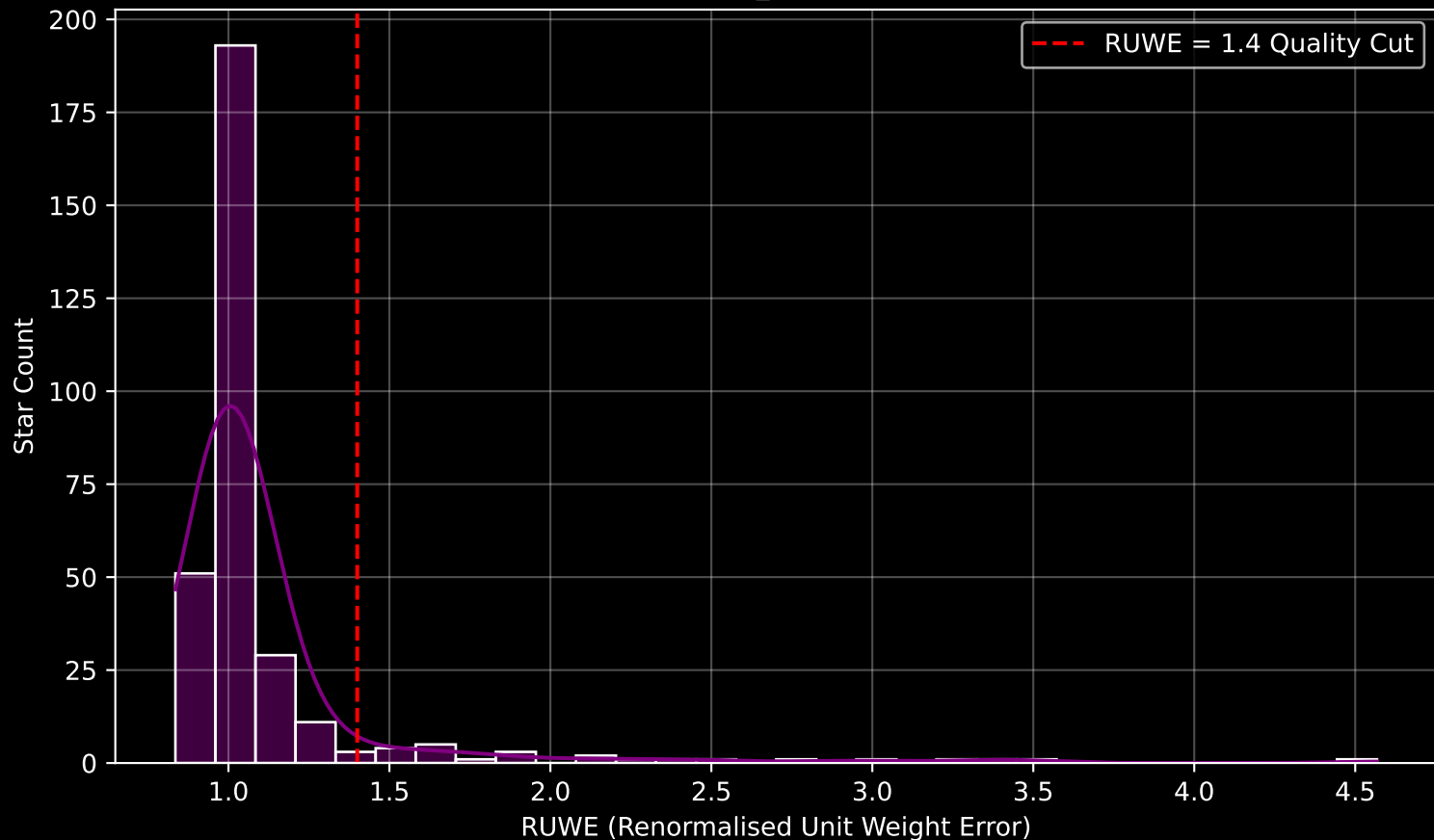
GAPOGEE DR17 Field [214+18_btx] RUWE Distribution (n= 311)
