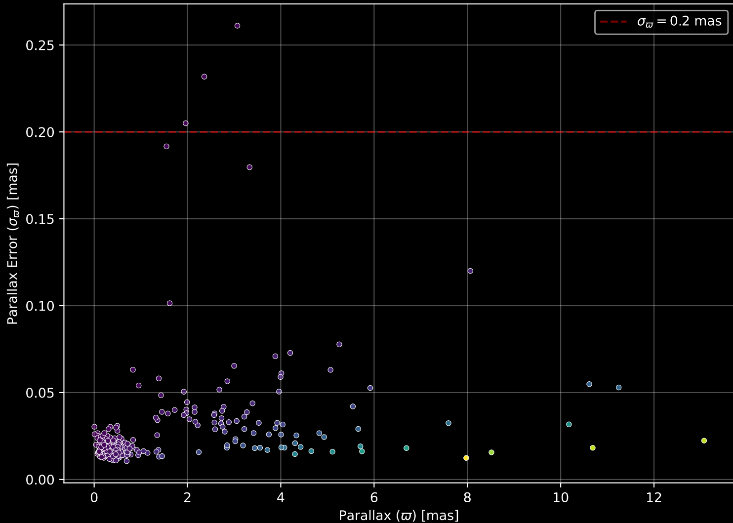
APOGEE DR17 Field: [214+18_btx] Parallax Quality (n= 319)
