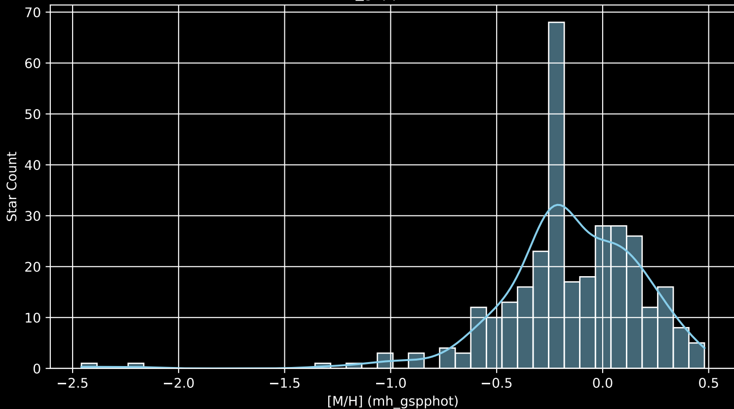
APOGEE DR17 Field: [214+18_btx [M/H] (mh_gspphot) (n= 317)
