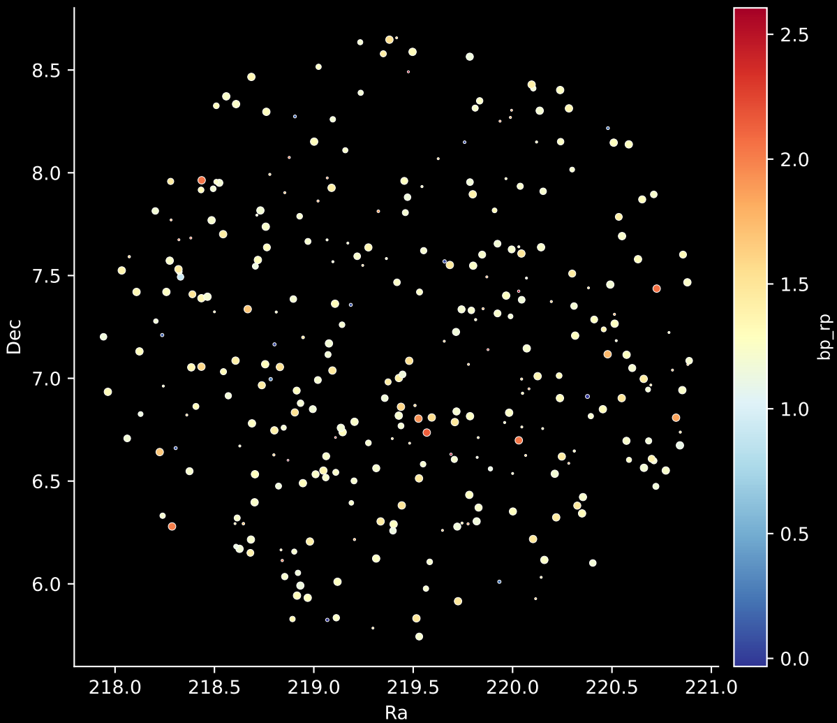
APOGEE DR17 Field: [214+18_btx] Stars: 319
