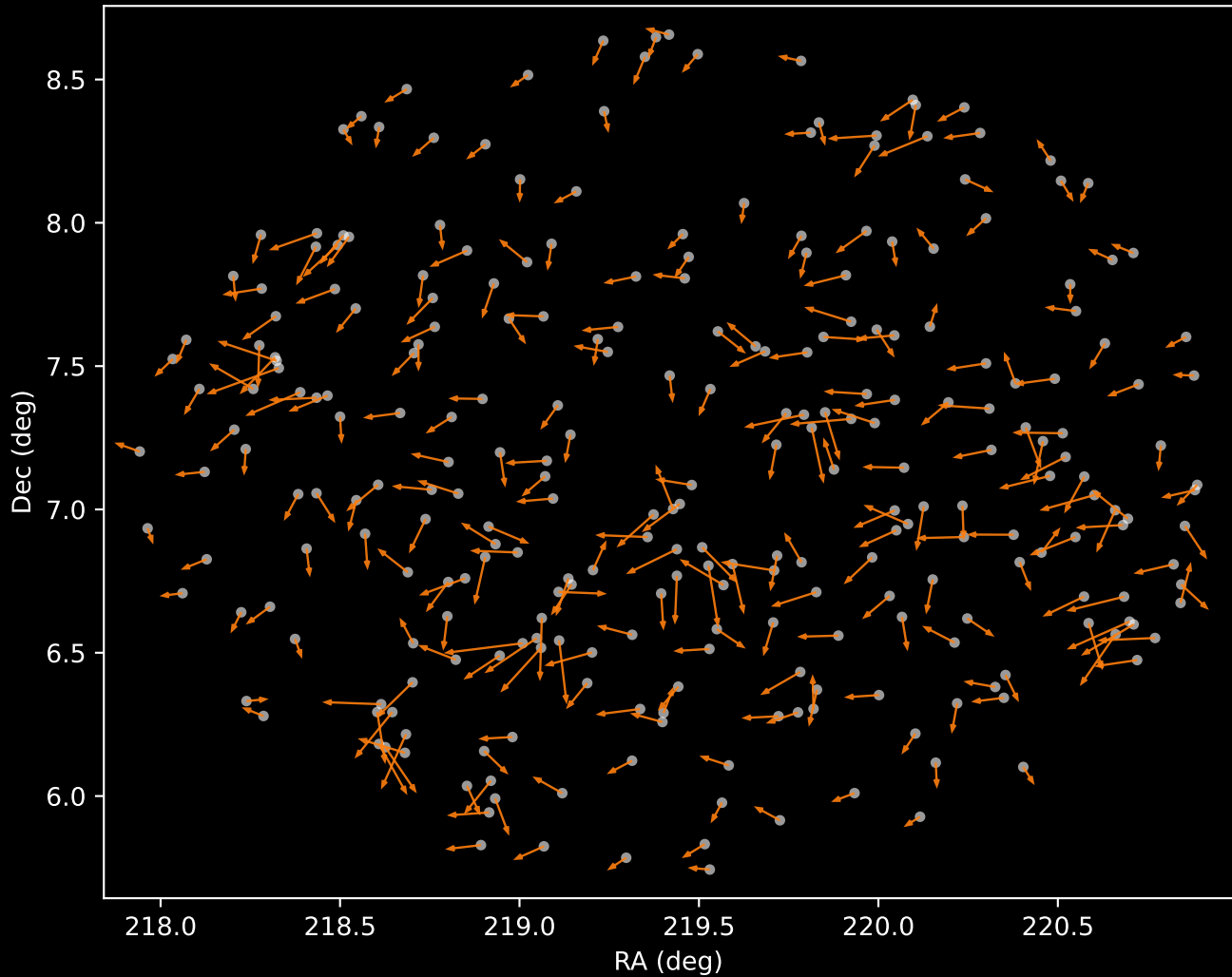
APOGEE DR17 Cluster 2 Proper Motion Vectors (n=273)
