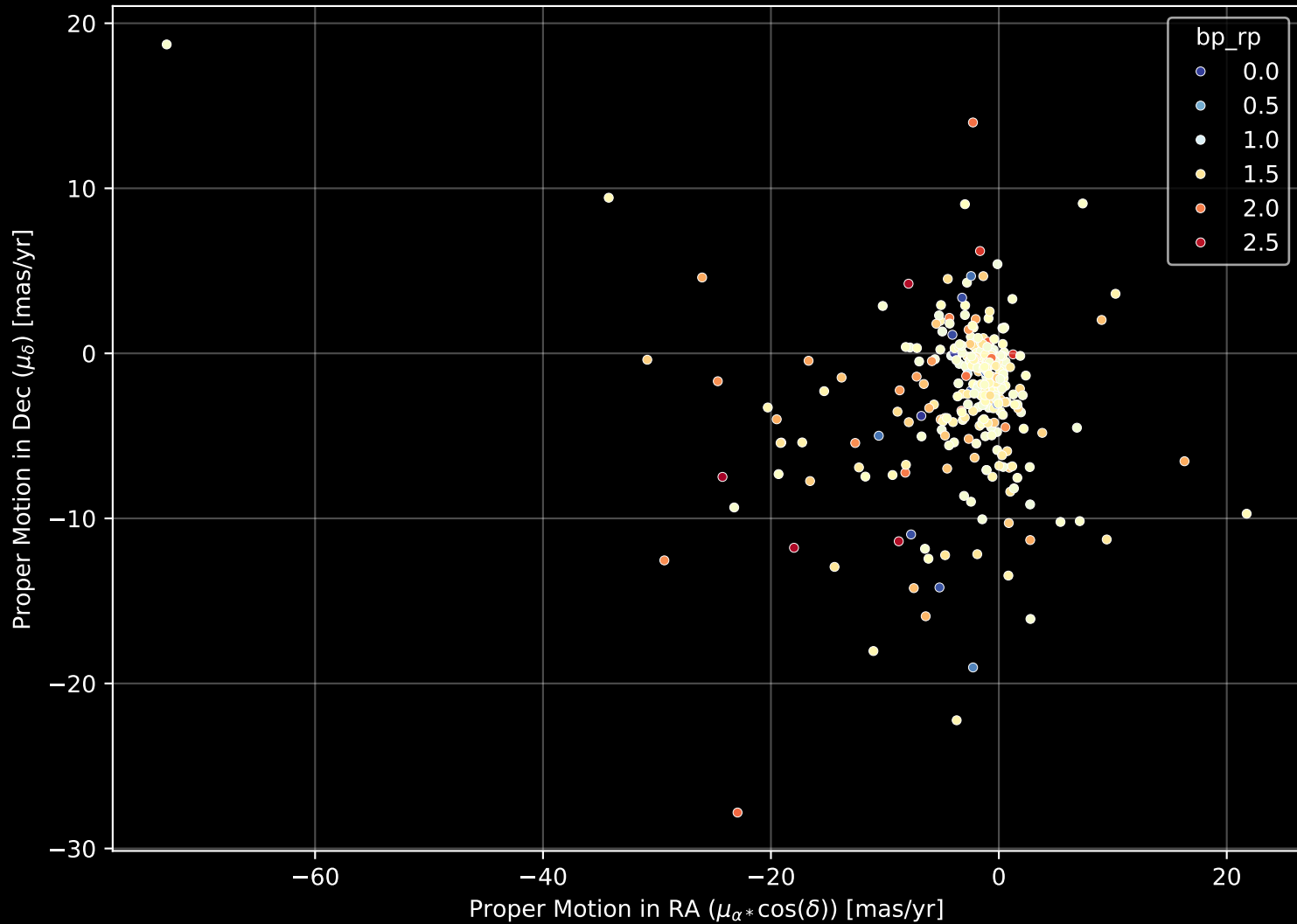
APOGEE DR17 Field: [214+18_btx] Proper Motion Diagram (n= 319)
